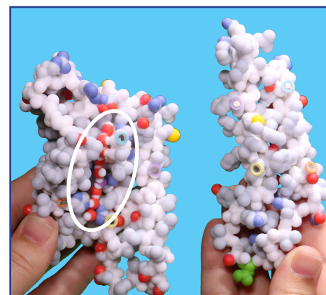
Water molecules passing through aquaporin
