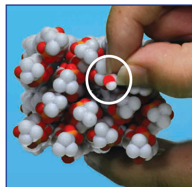
Passage of the water molecules.
